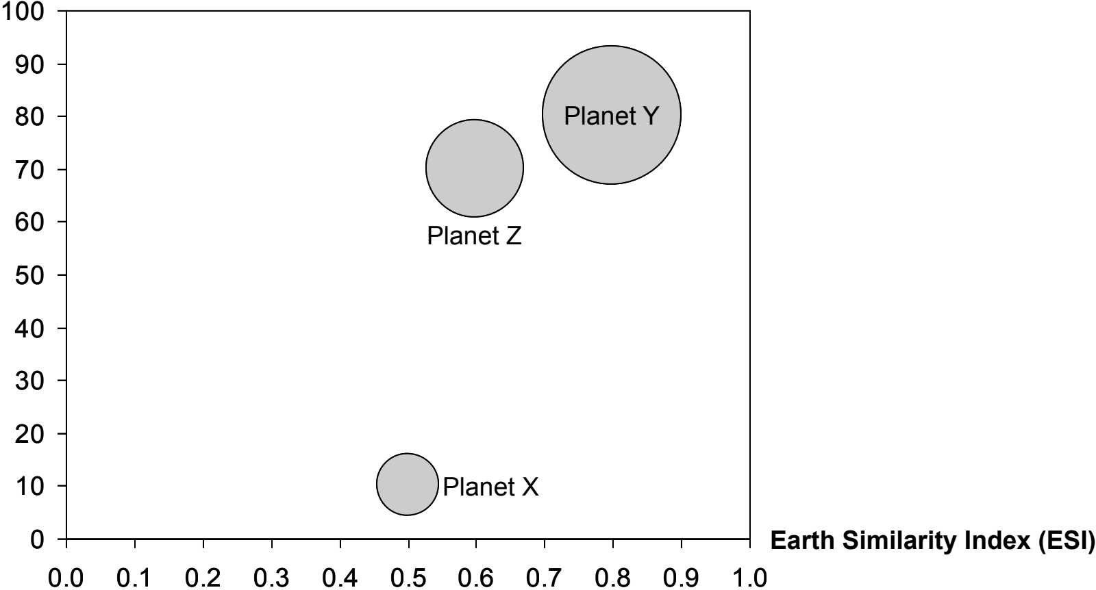
Percentile Location in Habitable Zone
